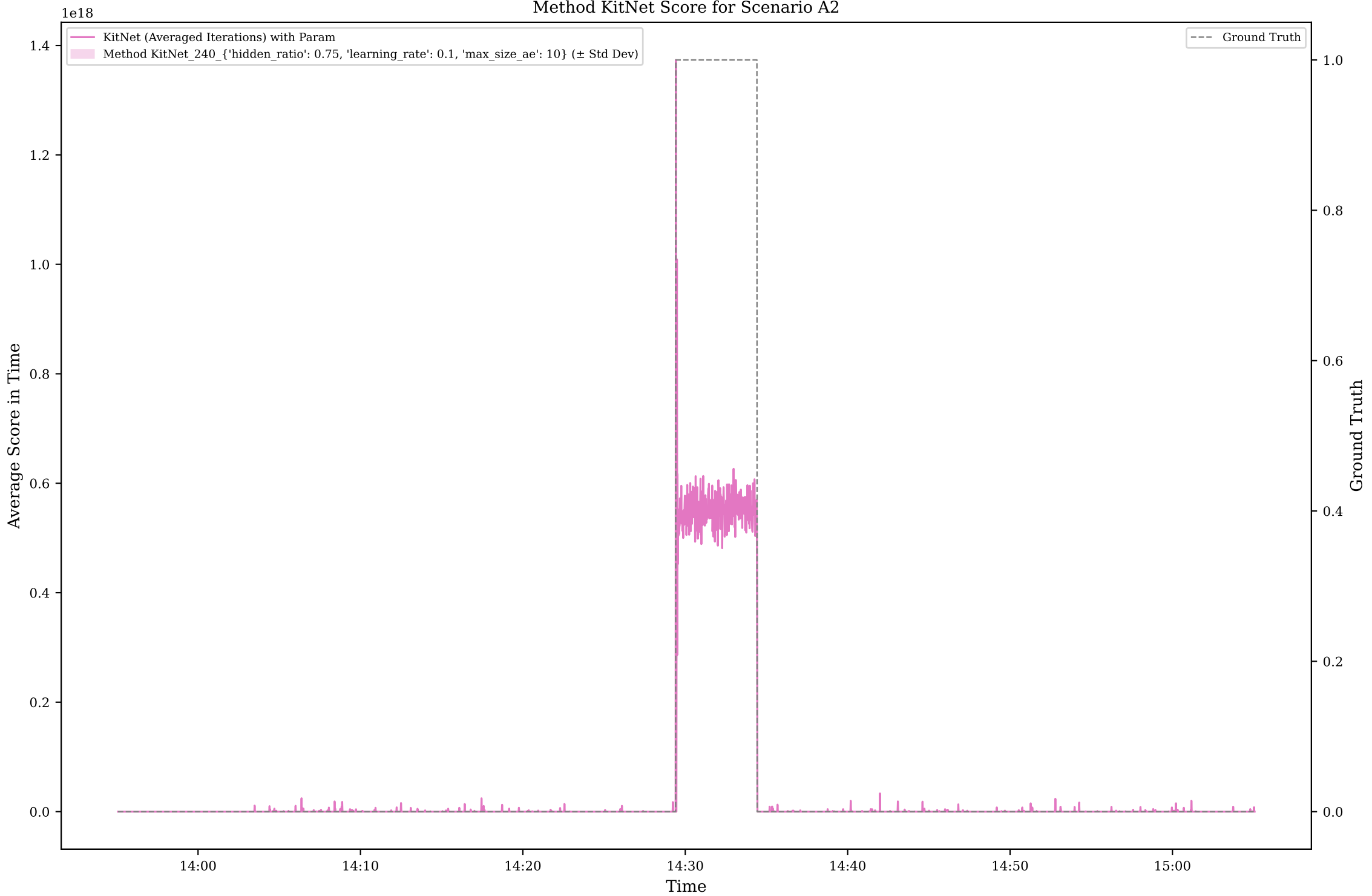
Method KitNet Score for Scenario A2
